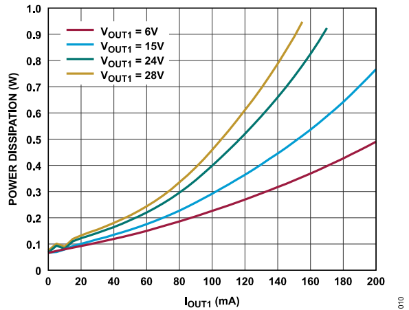
Figure 10. Power Dissipation at Various V_{OUT1} Output Voltages, T_A = 25^\circ\text{C} , V_{VINP} = 24\text{ V} , V_{OUT2} = 5.0\text{ V} , I_{OUT2} = 6\text{ mA} , V_{OUT3} = -15\text{ V} , I_{OUT3} = -4\text{ mA}
