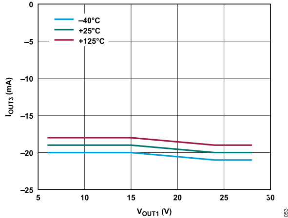
Figure 53. Inverting Regulator Maximum Output Current, V_{VINP} = 24\text{ V} , V_{OUT3} = -15\text{ V} , I_{OUT1} = 0\text{ mA} , I_{OUT2} = 0\text{ mA} , Based on Target of 70% I_{LIM} (FLYBACK) or I_{LIM} (INVERTER), Whichever Comes First
