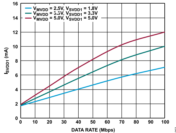
Figure 64. I_{SVDD1} vs. Data Rate at Various Supply Voltages, \overline{SSS} = \text{Low} , Clock Signal Applied on Single SPI Channel, Other Input Channels Tied Low
