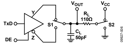
Figure 32. Driver Enable/Disable
