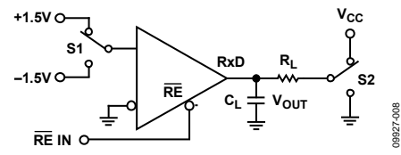
Figure 34. Receiver Enable/Disable
