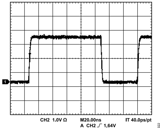
Figure 23. SYNC_OUT ( f_{\text{SYSCLK}}/384 )
