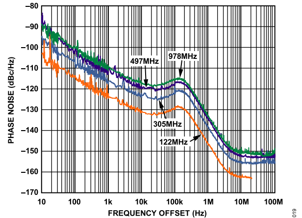
Figure 19. Absolute Phase Noise Curves of DDS Output Using Internal PLL at 2.5 GHz Operation
