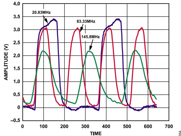
Figure 22. SYNC_CLK Waveform vs. Frequency ( f_{\text{SYSCLK}}/24 ), Measured at the SYNC_CLK Pin Using an Active Probe (1 GHz Bandwidth, 1 M \Omega , 1 pF) with the SYNC_CLK Pin Loaded by a 1 Inch PCB Trace Connected to an Open Subminiature Version A (SMA) Connector
