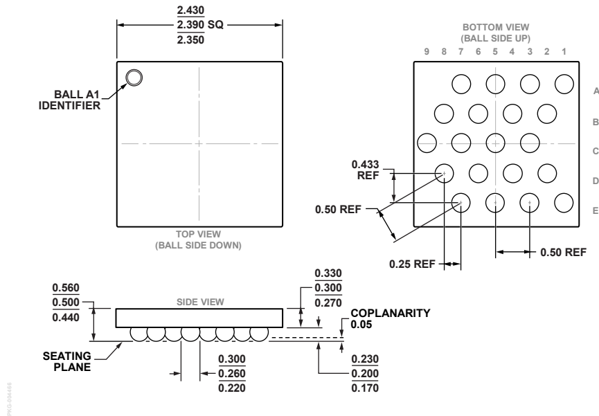
Figure 47. 20-Ball Wafer Level Chip Scale Package [WLCSF] (CB-20-12) Dimensions shown in millimeters
